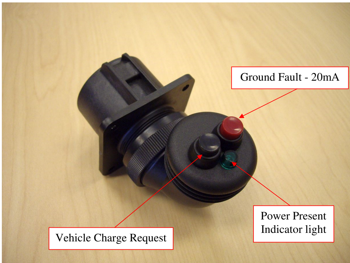
Figure 1: The CP-15 Tester
